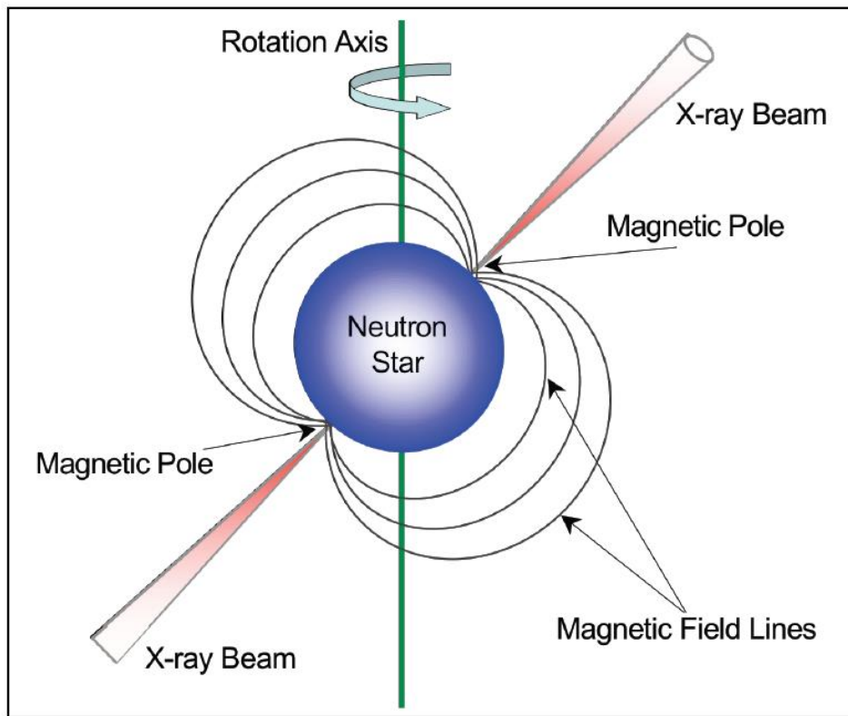
Figure 2-6. Diagram of pulsar with distinct rotation and magnetic axes.
